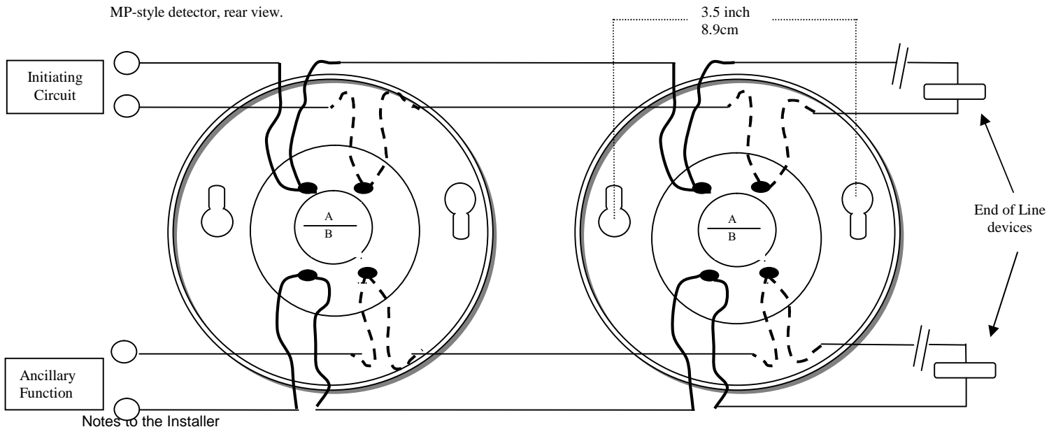
MP-style detector, rear view.
